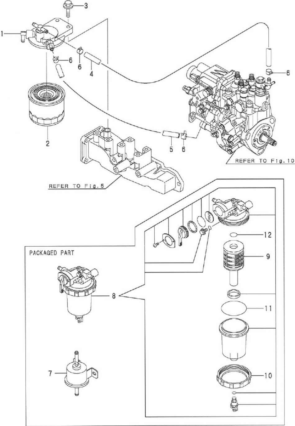
Y00V9800 Fig.12.FUEL PIPE
