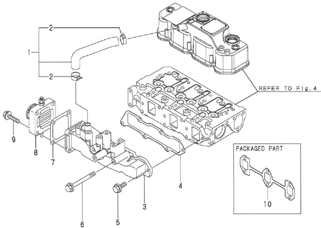
Y00V9800 Fig.5.SUCTION MANIFOLD
