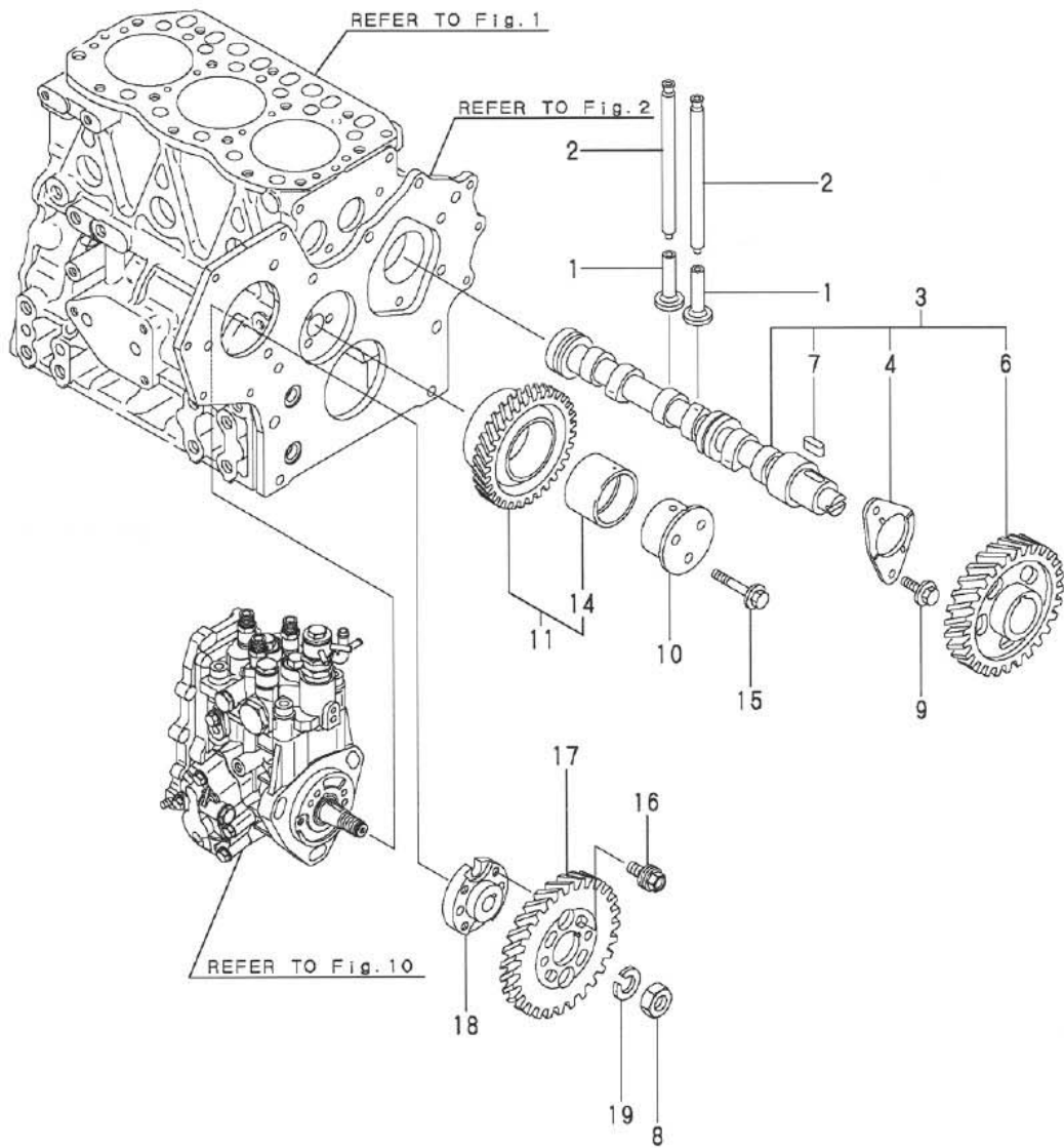
Fig.6.CAMSHAFT & DRIVING GEAR
