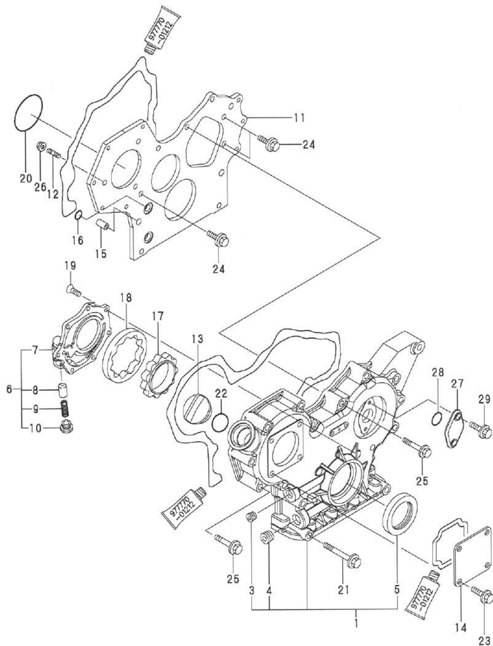
Fig.2.GEAR HOUSING
