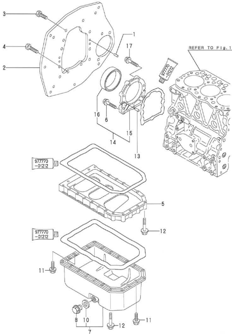
Fig.3.MOUNTING FLANGE & OIL SUMP
