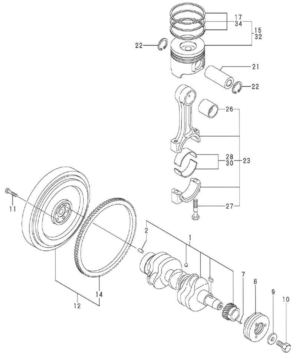
Fig.7.CRANKSHAFT & PISTON
