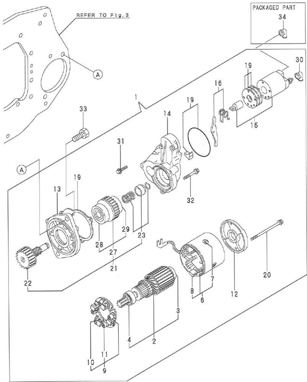
Fig.13.STARTING MOTOR
