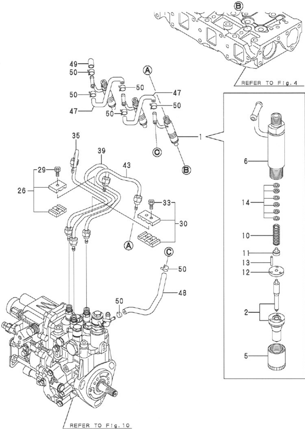
Fig.11.FUEL INJECTION VALVE
