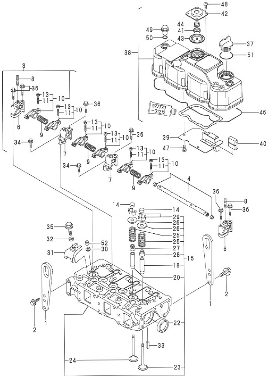
Fig.4.CYLINDER HEAD & BONNET
