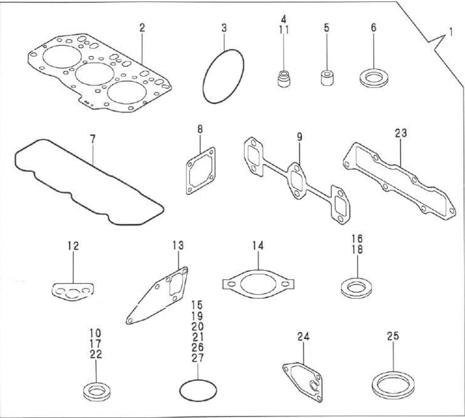
Fig.15.GASKET SET & TOOLS
