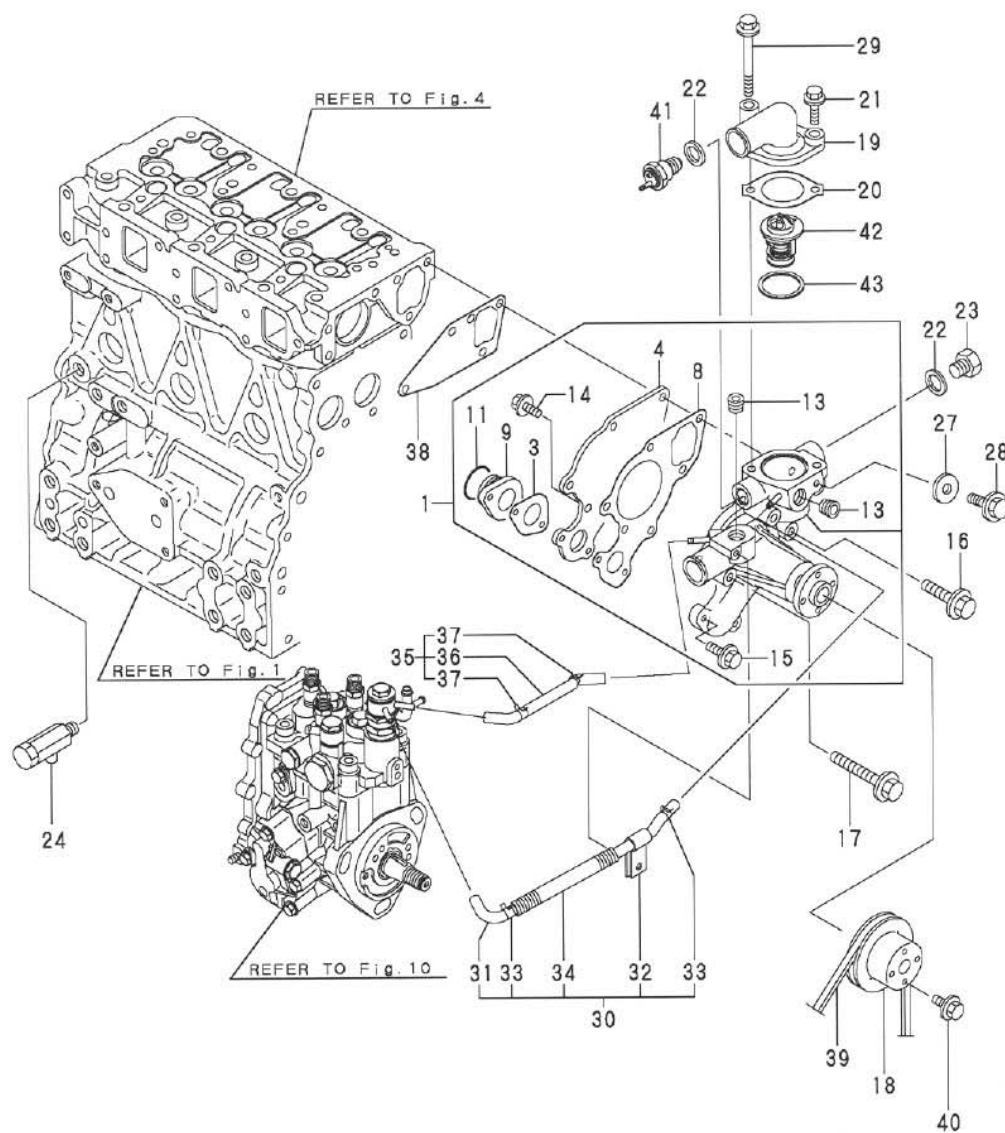
Fig.9.COOLING WATER SYSTEM
